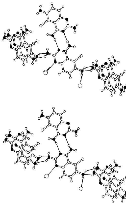
Fig. 2. Stereoscopic view of the hydrogen-bonding environment of one TCQ molecule. Atomic vibrational ellipsoids are scaled to the 30% enclosure level, except those for the H atoms, which are represented by spheres of a fixed arbitrary radius. N atoms are denoted by filled circles. This view is along the a direction with a horizontal and c approximately vertical.
